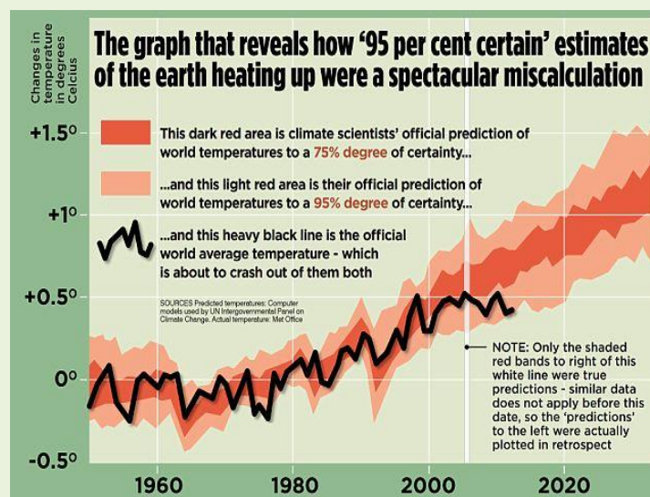
Rising CO 2 levels are not causing world mean global temperature to rise.
